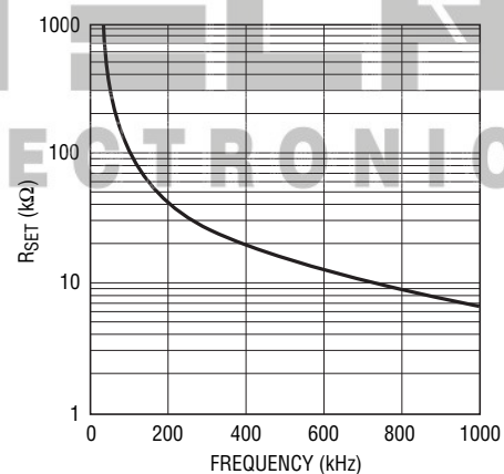
Figure 7. Timing Resistor ( R_{SET} ) Value
